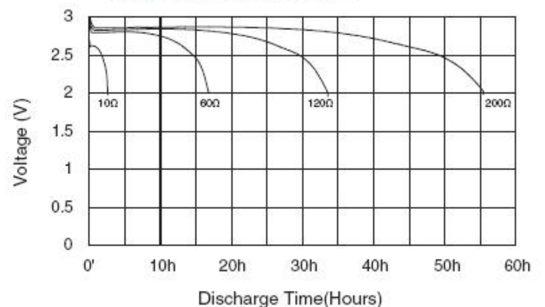
Continuous Discharge at 23°C
