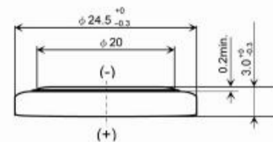
Dimension Drawing
