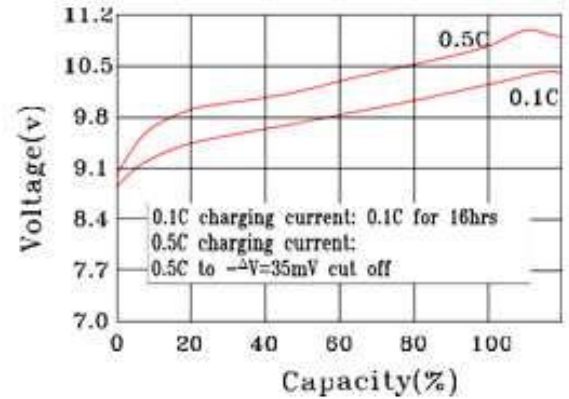
CHARGE CHARACTERISTICS
